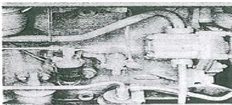
Illustr. 25A Engine driven 9 g.p.m. hydraulic pump.
