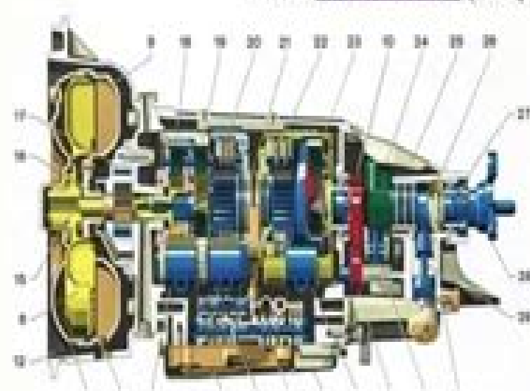
Fig. 1 4-speed transmission with fluid coupling
