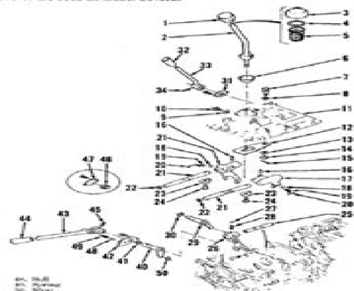
Fig. 73—Exploded view of shifter mechanism used on Models 853000 and 851000. Components 33 through 44 are used on Model 851000 and components 45 and 47 are used on Model 853000.
