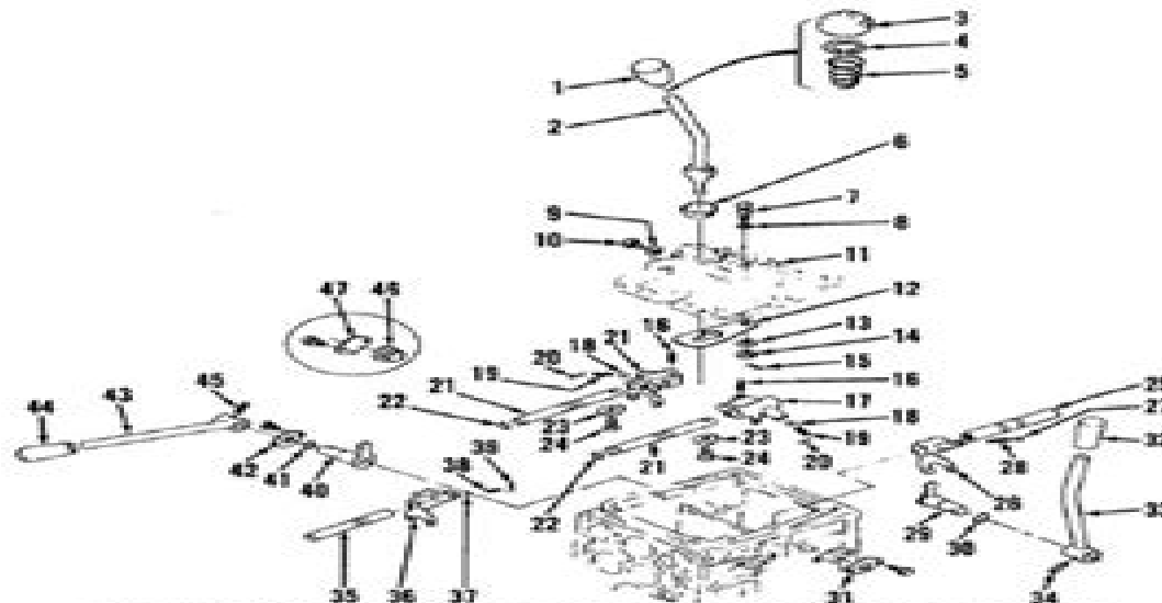
Fig. 73—Exploded view of shifter mechanism used on Models 853000 and 851000. Components 33 through 44 are used on Model 851000 and components 45 and 47 are used on Model 853000.
