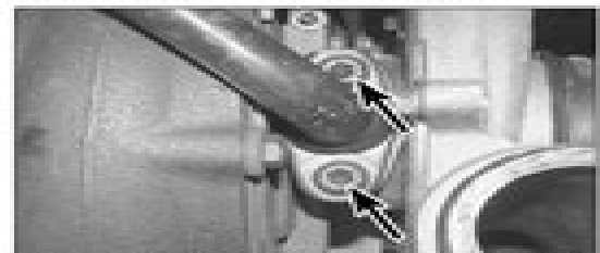
13.10a Undo the 2 Torx bolts (arrowed) securing the oil return pipe to the turbocharger ...
