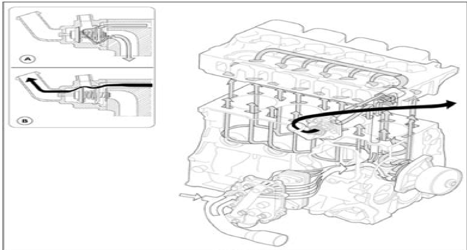
FIGURE 1 ENGINE COOLING SYSTEM DIAGRAM
