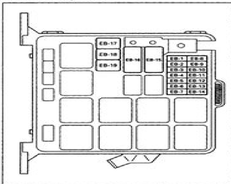
Fuse Box
