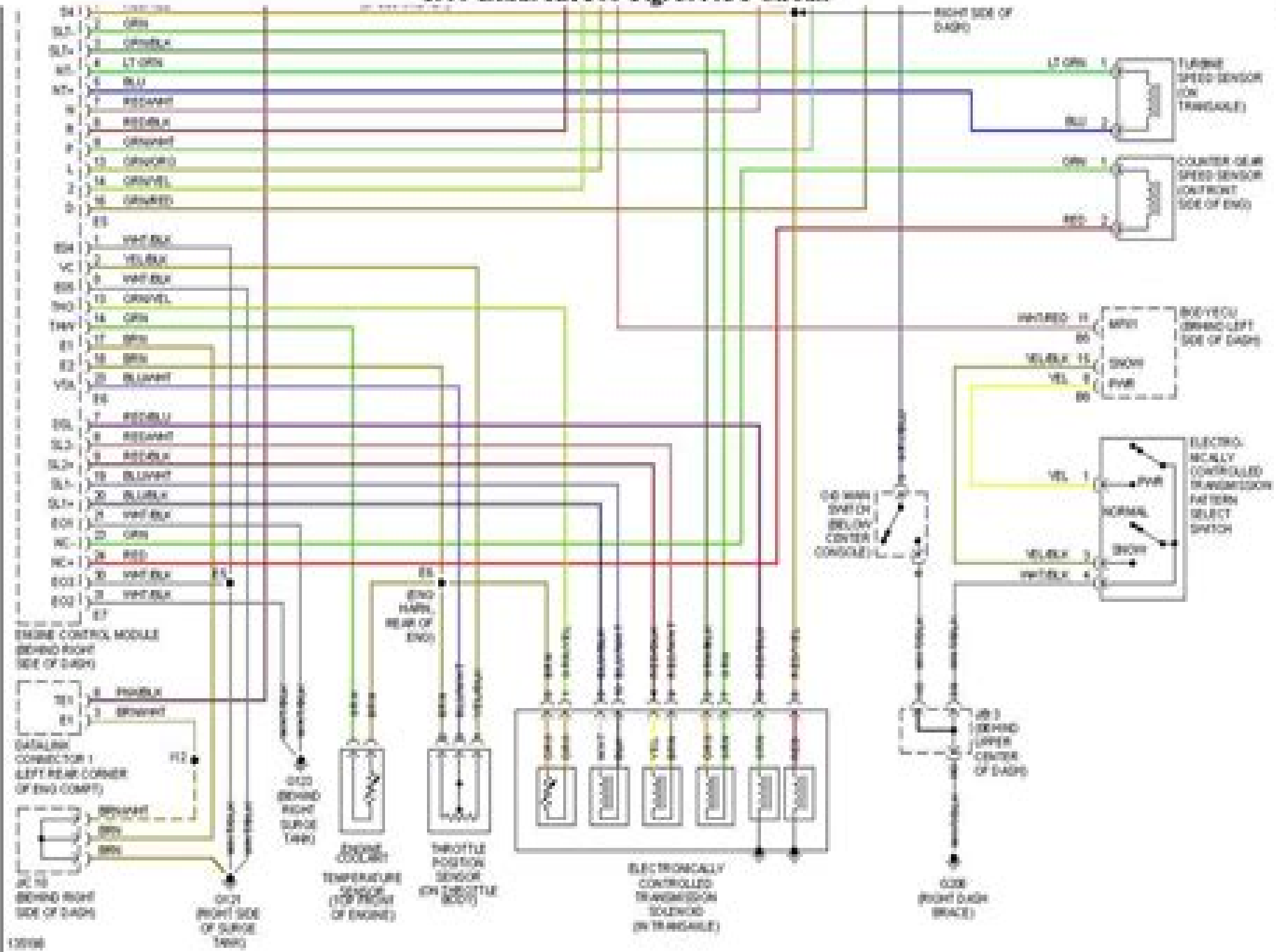
1999 Lexus RX 300- Fig. 59: AT Circuit
