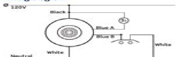
ODC05-I; Wiring Diagram with optional switch for override to OFF * Same wiring for all voltages.
