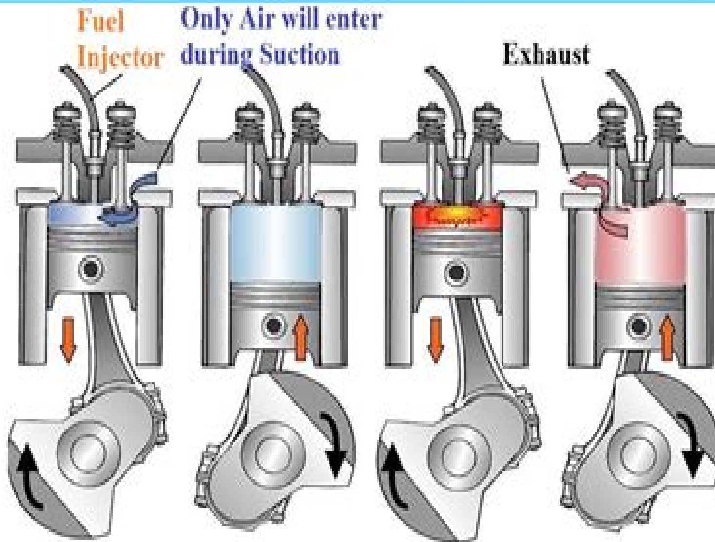
Suction Compression Expansion Exhaust
