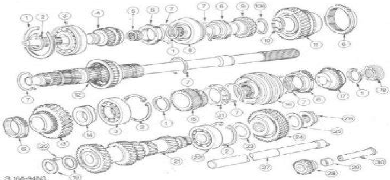
Fig.112. 'W' Transmission - gearbox shafts.
