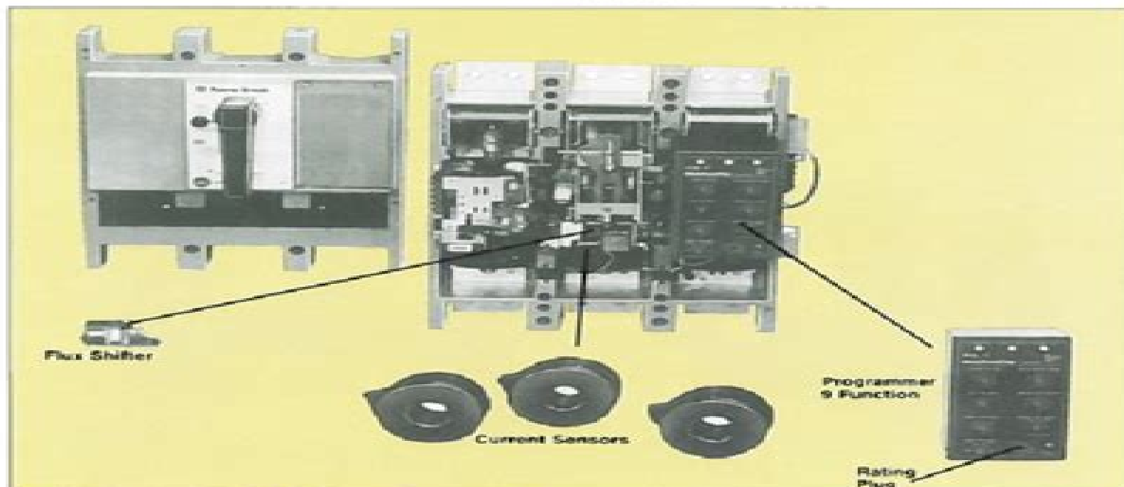
Fig. 10.1 MicroVersaTrip RMS-9 System Components
