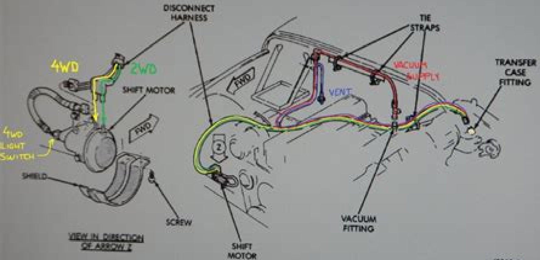
Fig. 10 Vacuum Hose Routing
