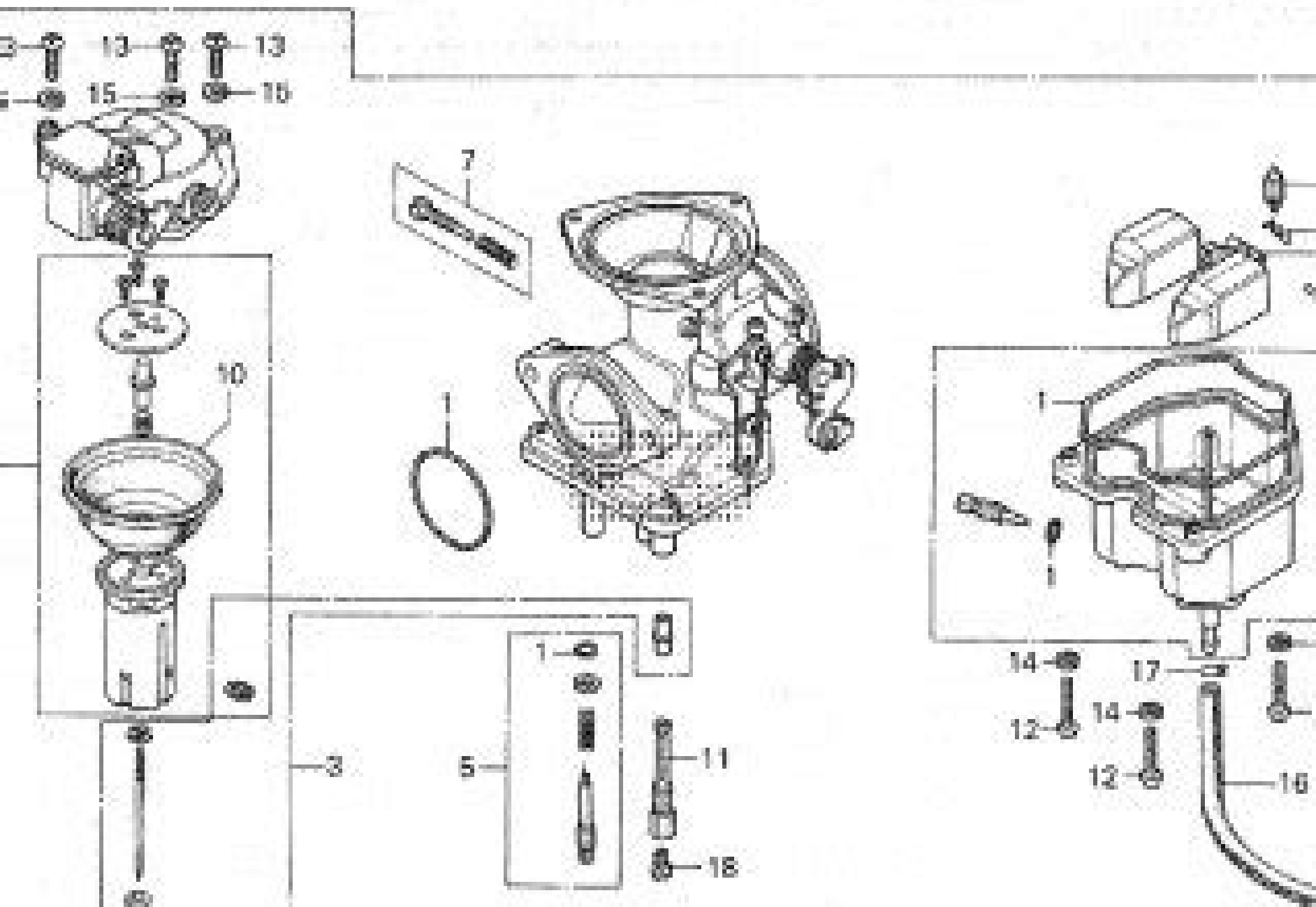
E-1 CARBURETOR (CD 125T)
