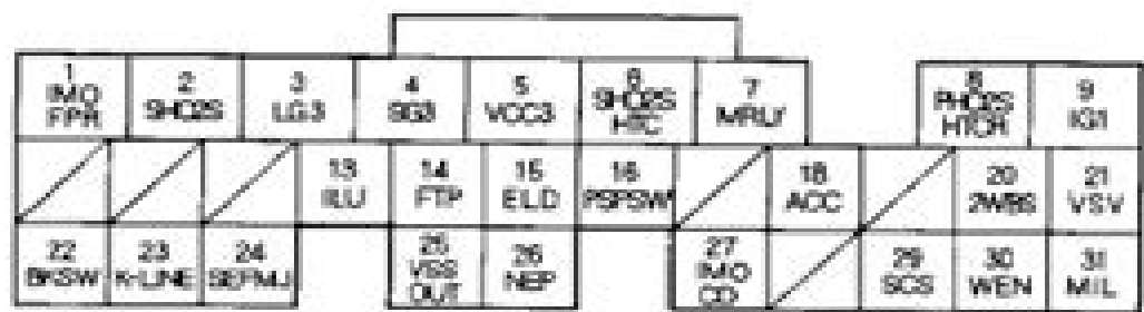
Wire side of female terminals
