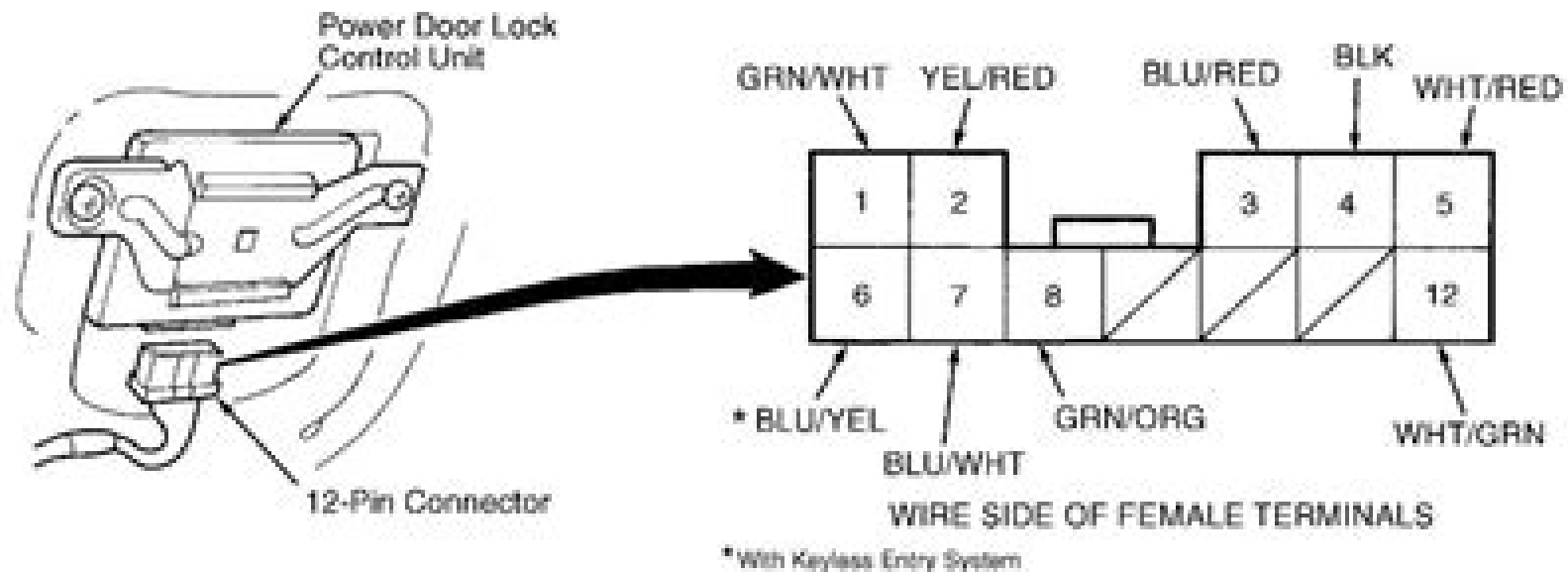
Fig. 5: Power Door Locks Control Unit Input Test (Without Keyless Entry) Courtesy of AMERICAN HONDA MOTOR CO., INC.
