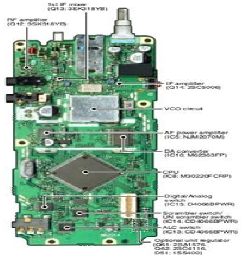
Bottom view
