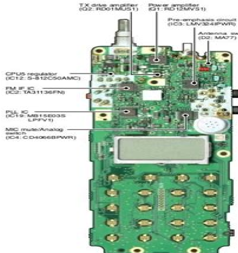
Top view
