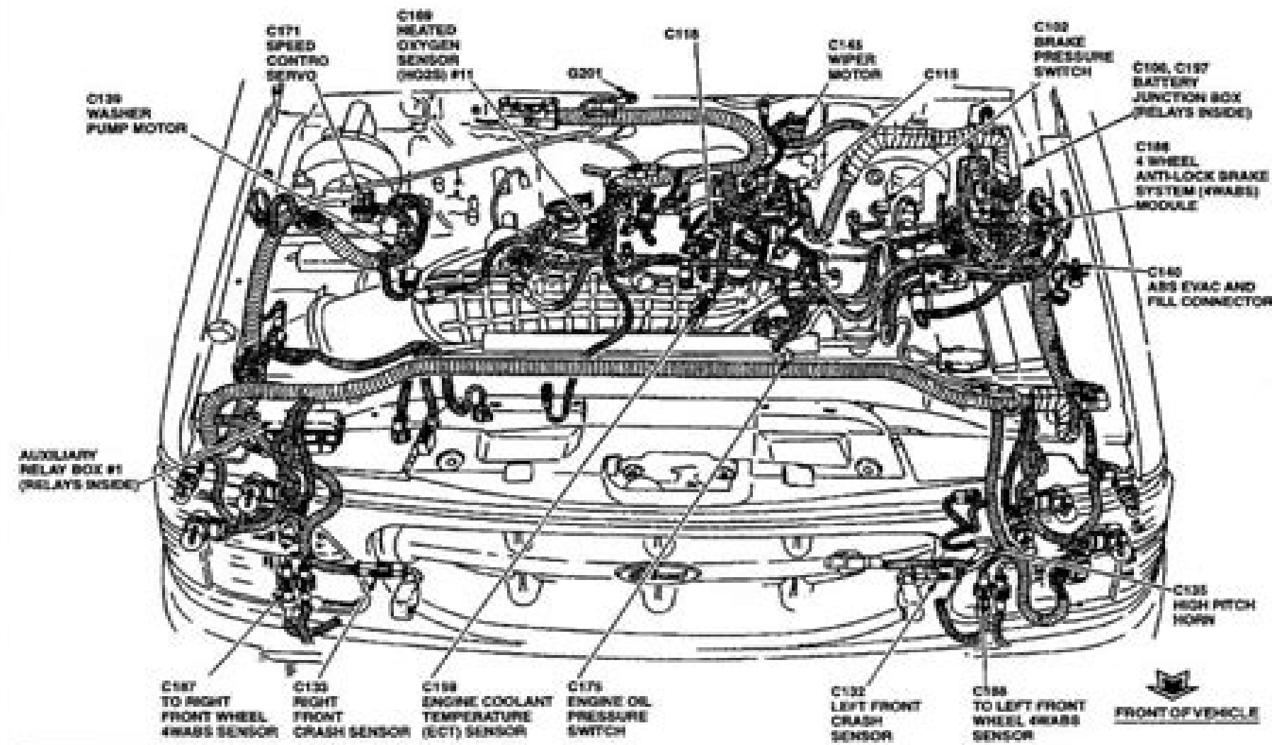
Fig 1: Engine Compartment (4.0L - DOHC)
