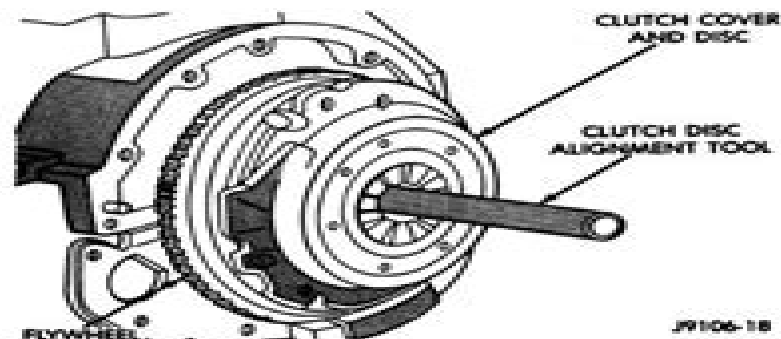
Fig. 3 Typical Method Of Aligning Clutch Disc
