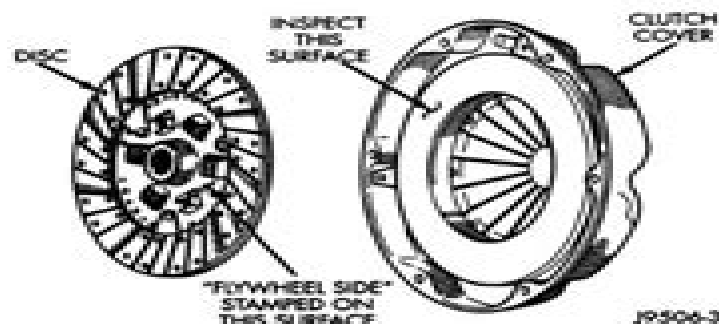
Fig. 2 Clutch Disc And Pressure Plate Inspection
