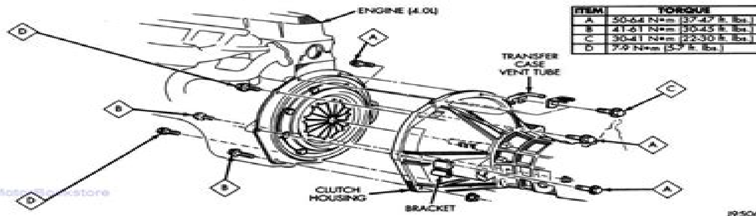
Fig. 4 Manual Transmission Mounting (4.0L)
