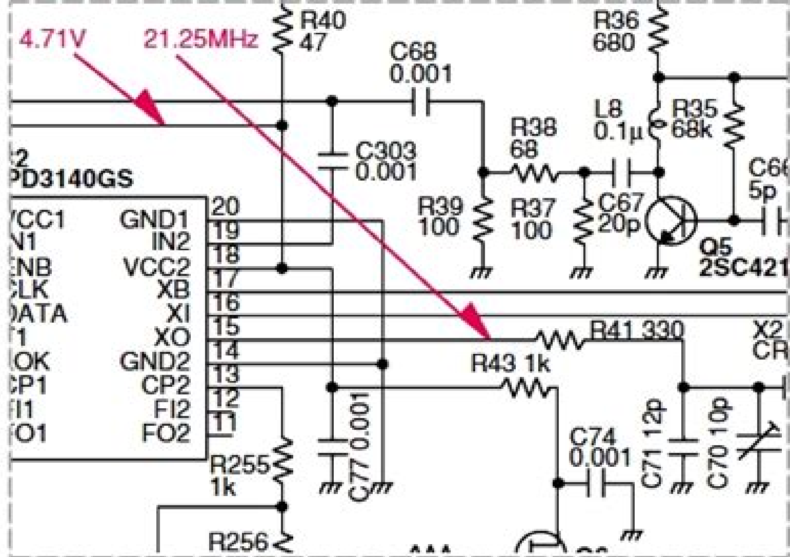
Preview: ICOM IC-M502 schematic diagram
