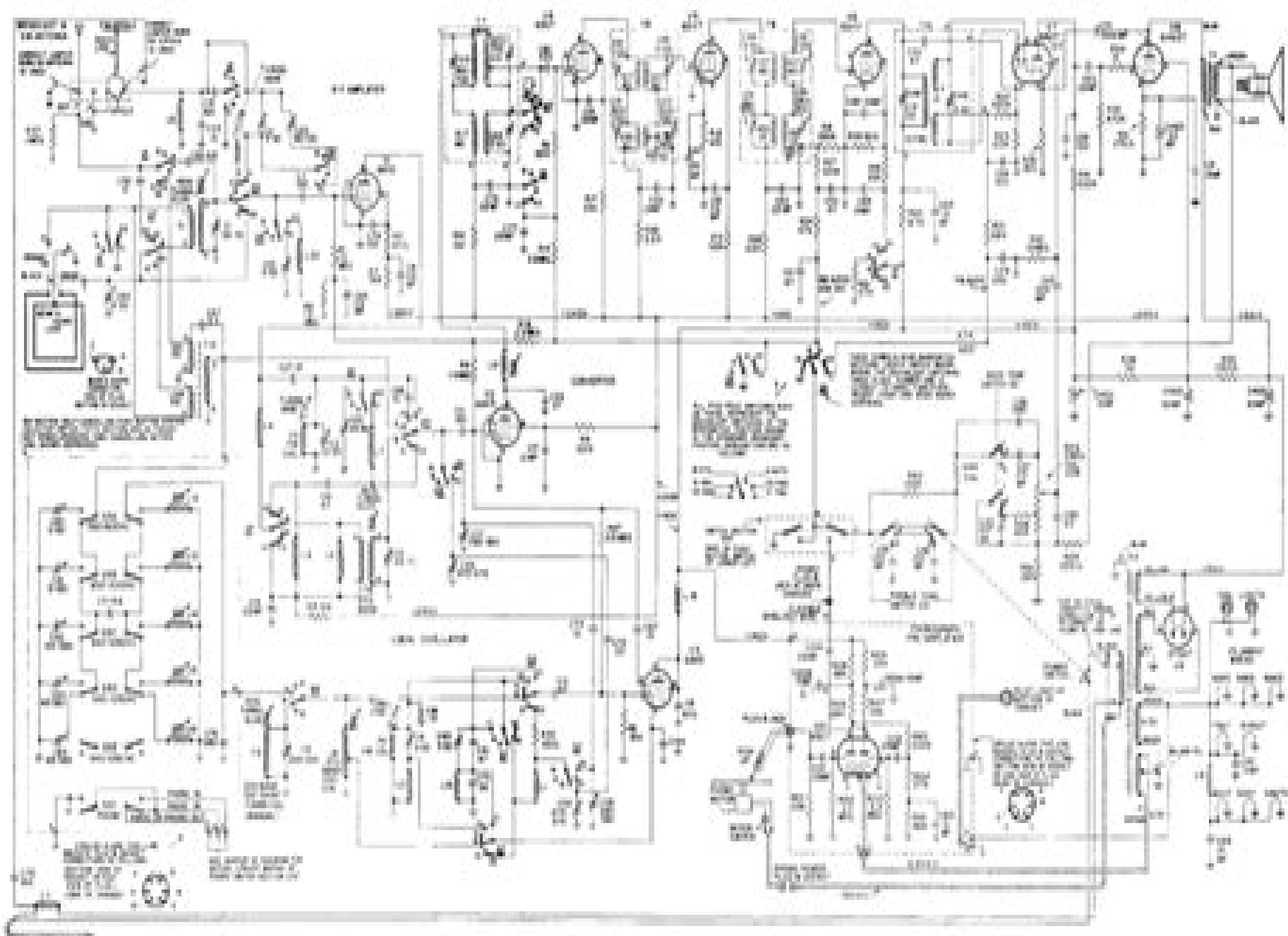
General Electric Model 417-A Radio Photograph (ca. 1947)
