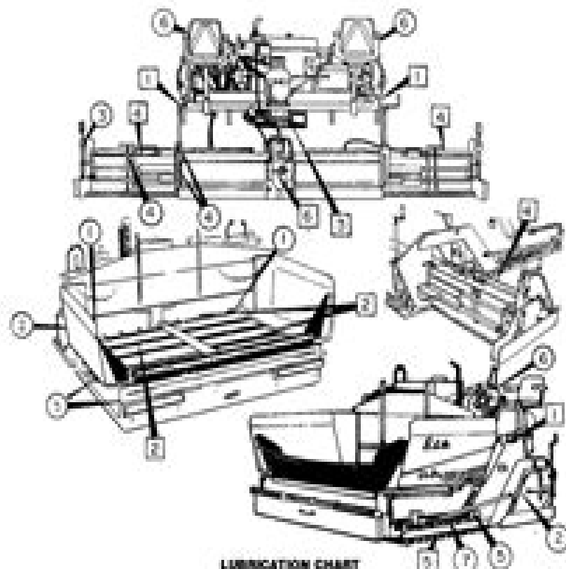
LUBRICATION CHART
