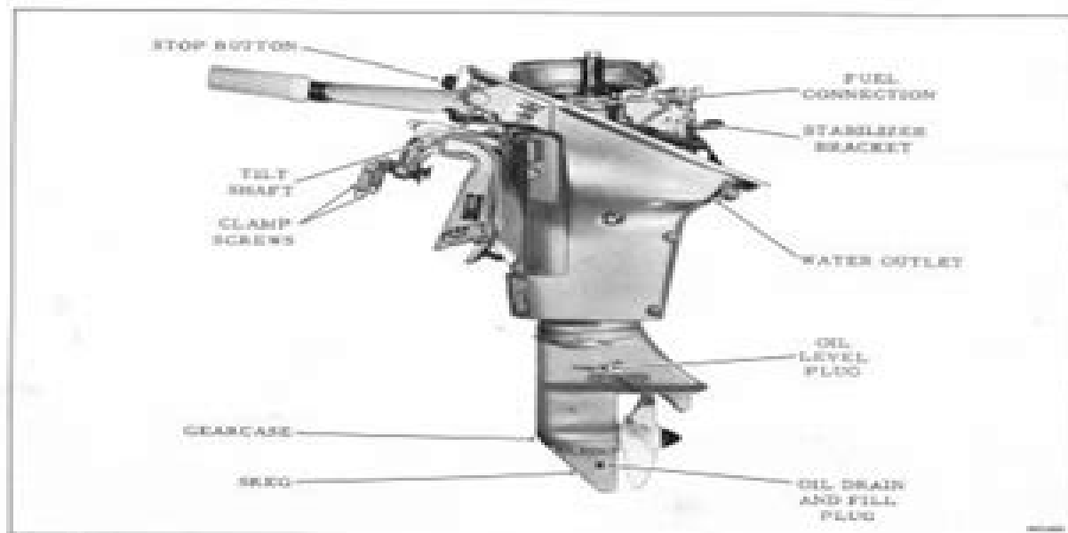
Figure 1-2, Port Side
