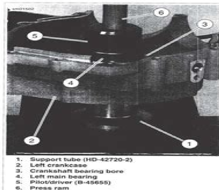
Figure 3-81. Installing Left Main Bearing in Crankcase
