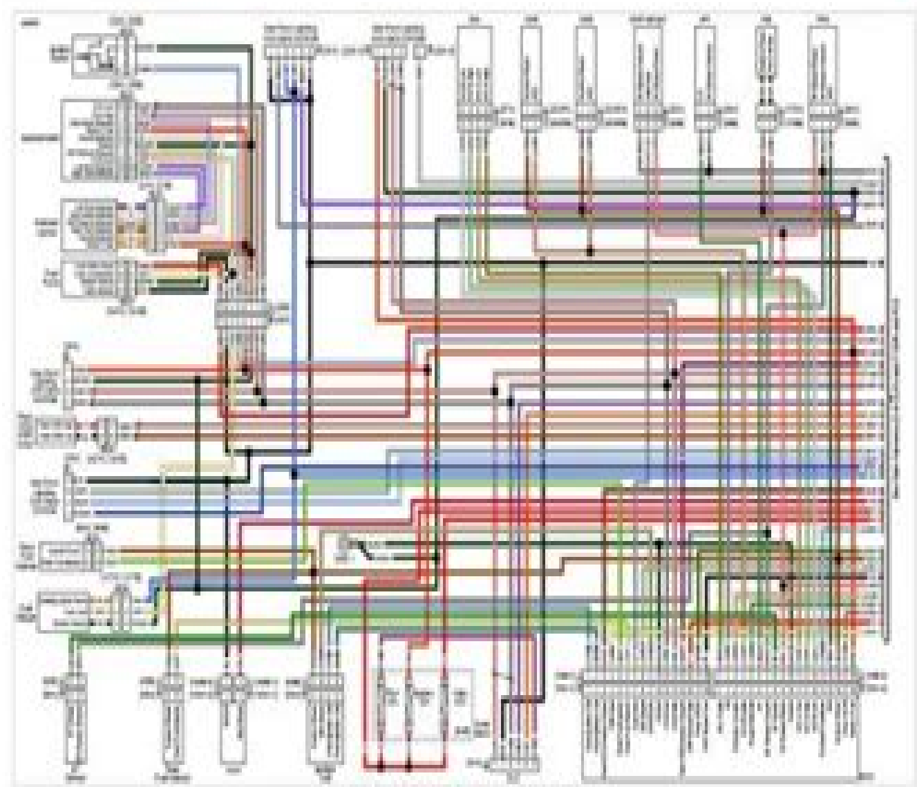
Figure 1-1. Main harness wiring diagram (engine front view)
