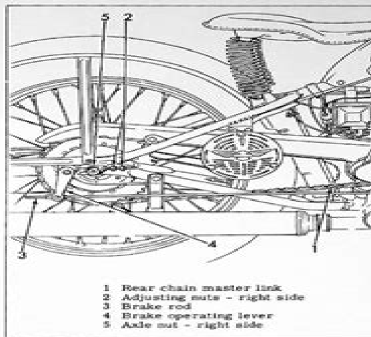
Figure 2C-22. Rear Wheel
