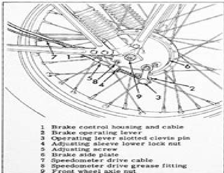
Figure 2C-21. Front Wheel
