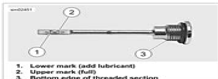
Figure 1-18. Filler Plug/Dipstick
