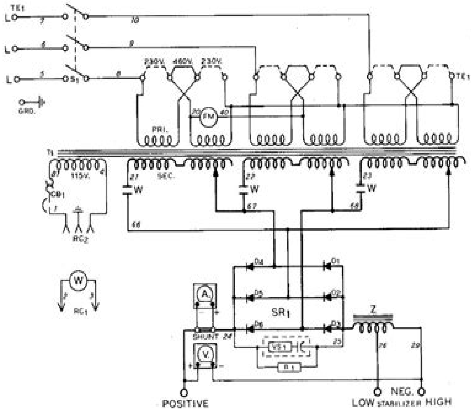
Circuit Diagram No. CA-901 851-1A
