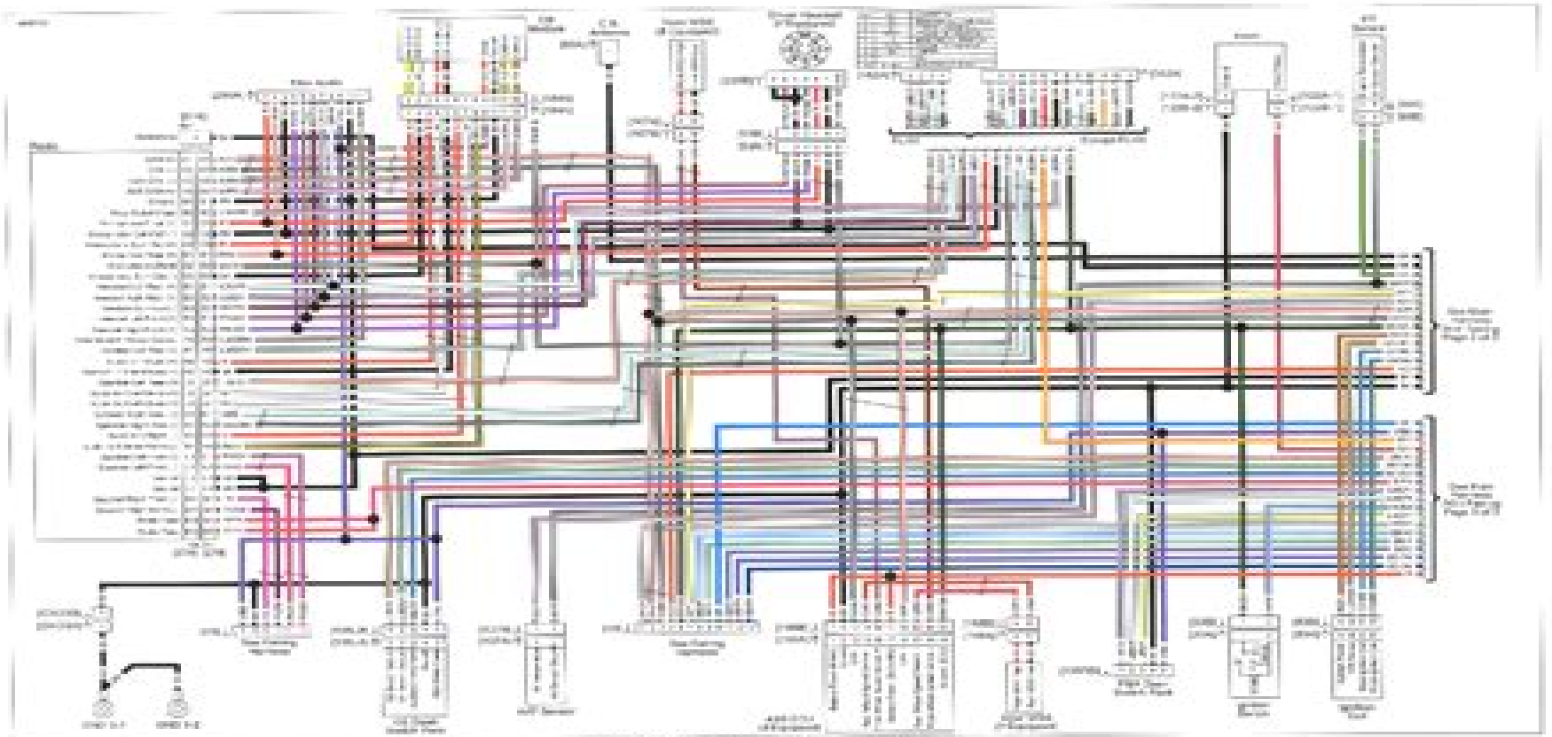
Figure 2-15: Main Harness (1 of 2) (Wire Numbering)
