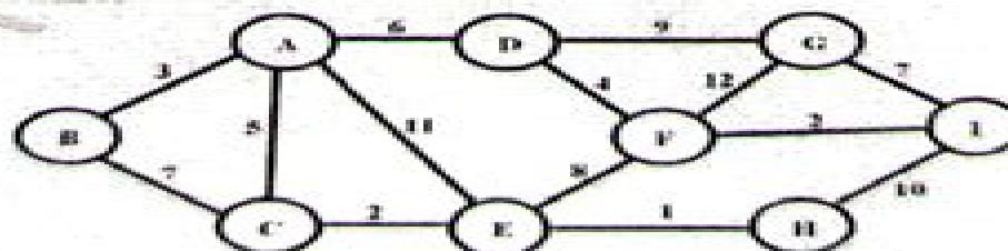
Graph G(V,E)
