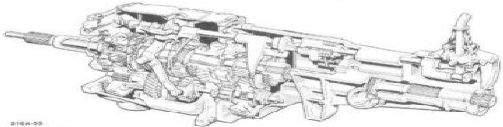
Fig.111. 'N' Transmission.
