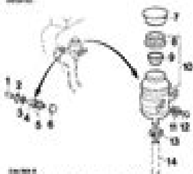
Fig. 5 - Brake Fluid Reservoir, Combines with Four-Speed Transmission
