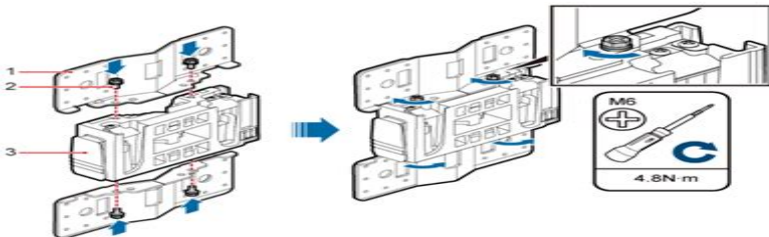
Figure 7-17 Installing the adapting plate assembly
