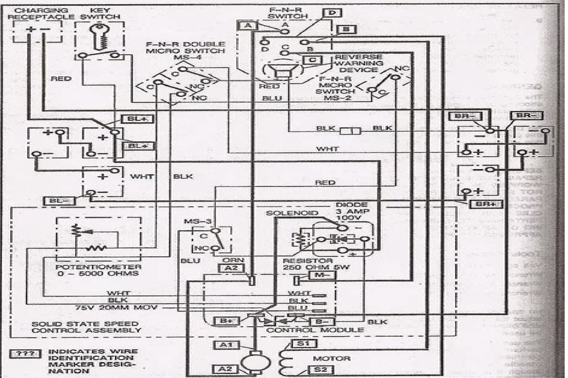
FIG. N-3 POWER WIRING DIAGRAM
