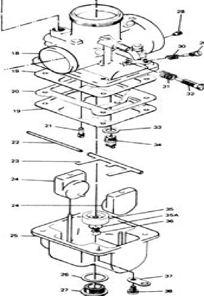
DIAGRAM A Exploded view of a SPIGOT MOUNT TYPE MIKUNI CARBURETOR
