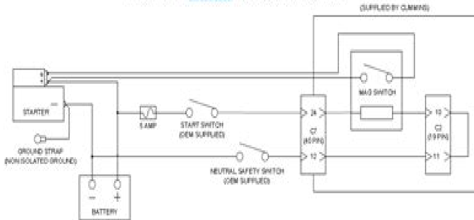
Figure 7: Neutral Safety/Start Circuit
