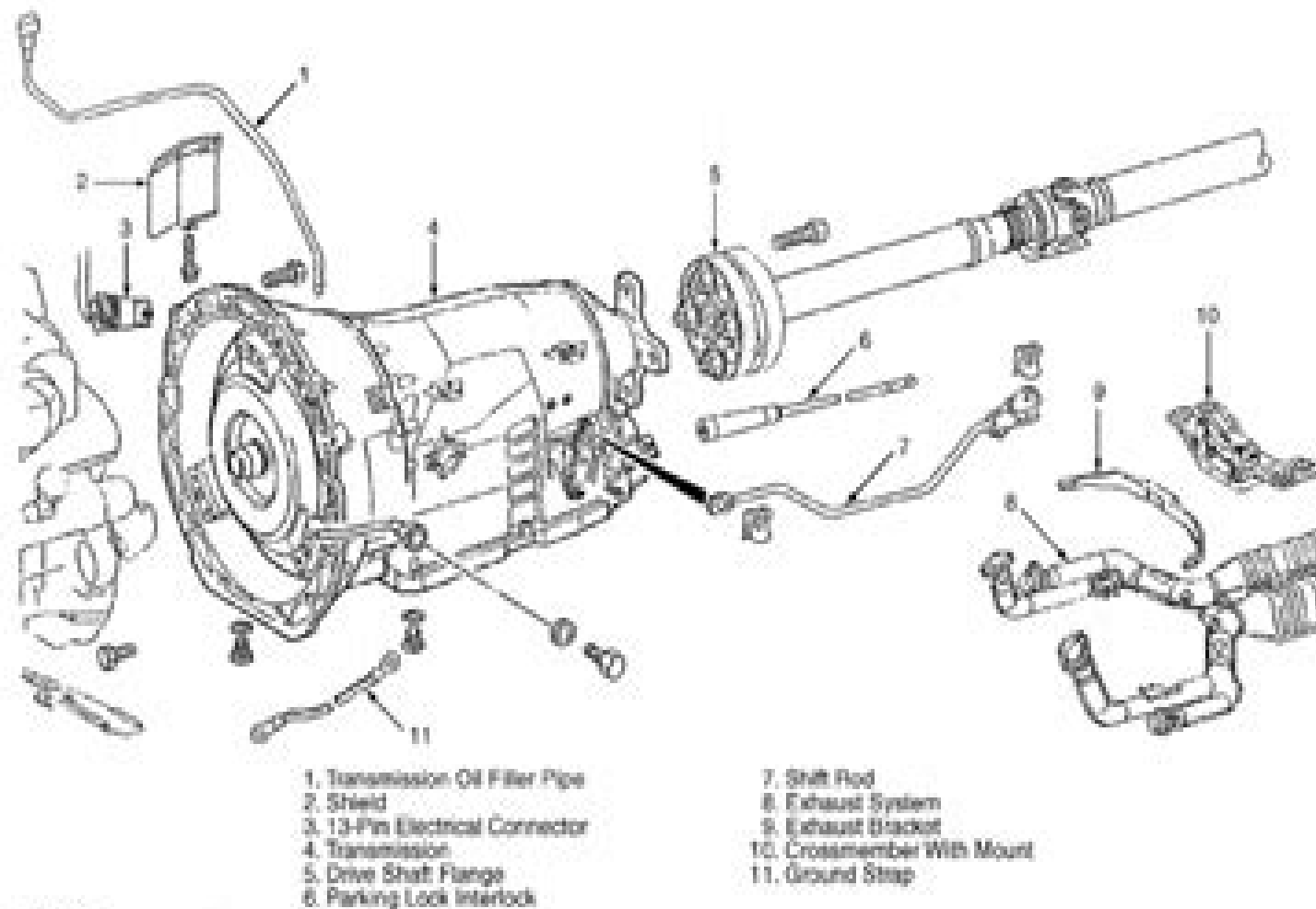
Fig. 1: Removing & Installing Transmission (Typical) Courtesy of Mercedes-Benz of North America.
