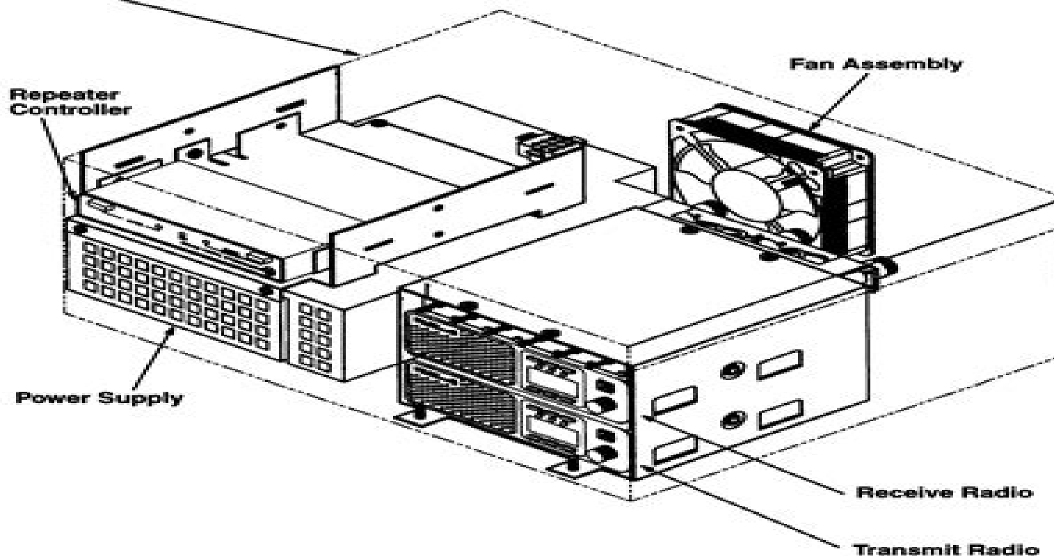
Figure 1-2. GR500 Repeater Station (before mounting)
