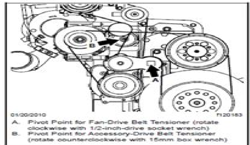
Fig. 2, Releasing the Tensioners
