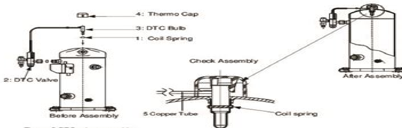
Figure 2 DTC valve assembly
