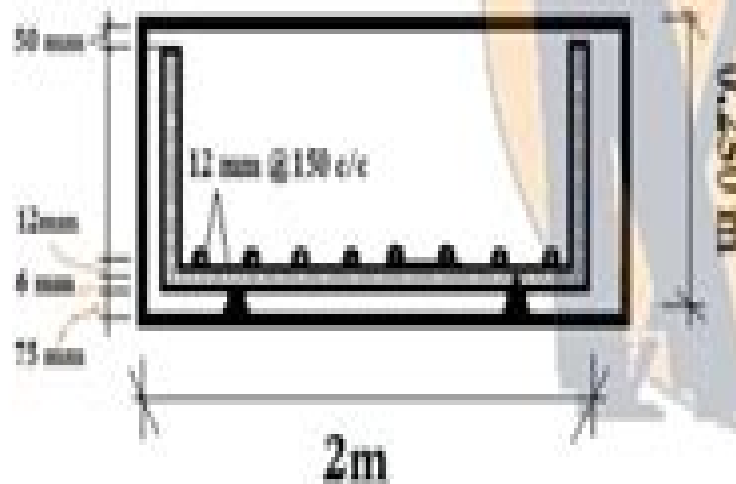
x-Section AA
