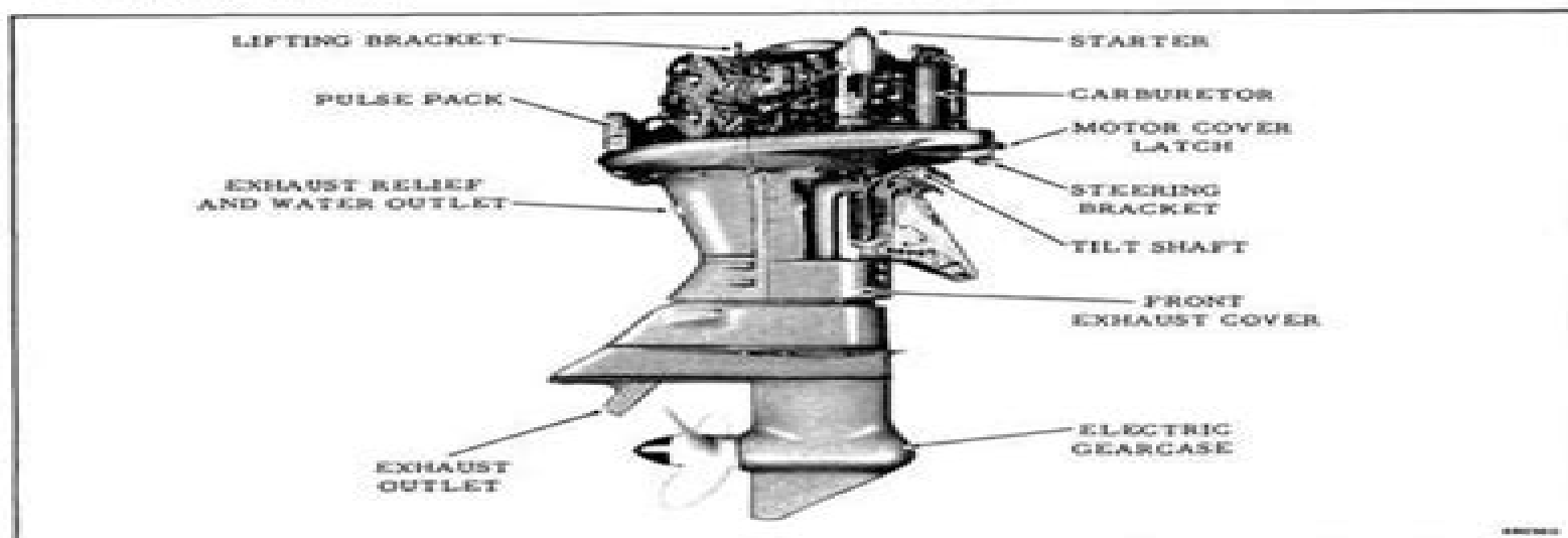
Figure 1-1. Starboard Side
