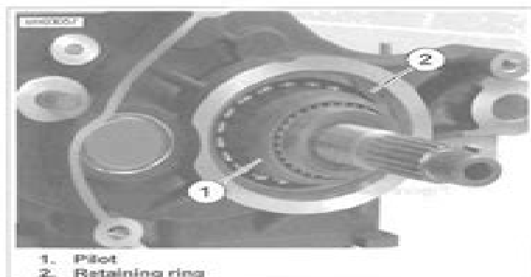
Figure 6-45. Install Pilot
