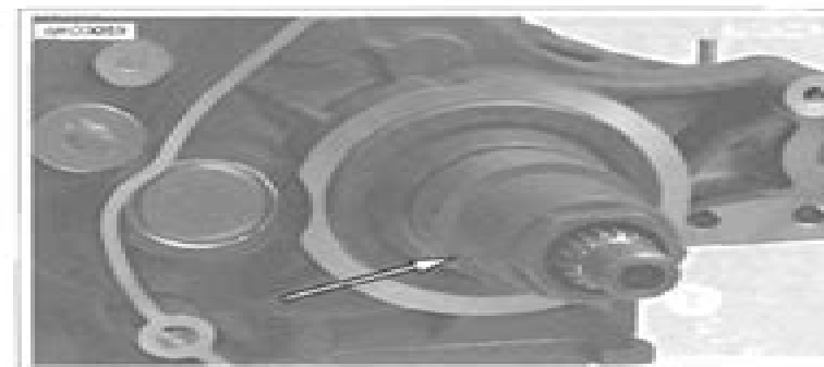
Figure 6-47. Install Adapter
