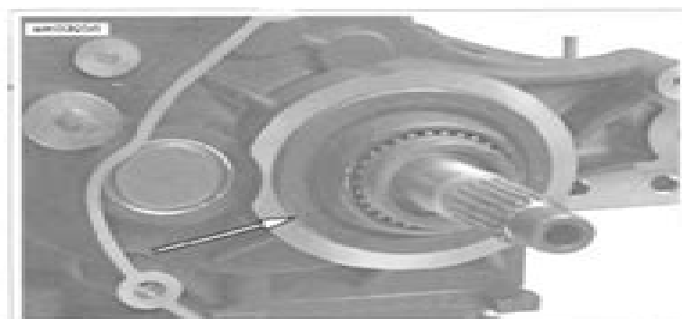
Figure 6-46. Place Main Drive Gear Seal Over Pilot
