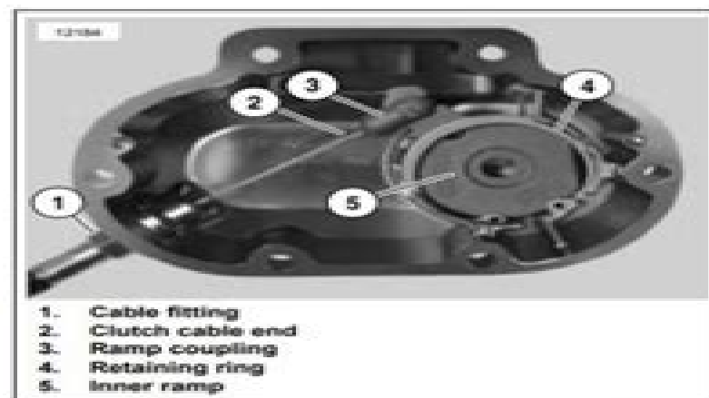
Figure 2-101. Clutch Cable Connection
