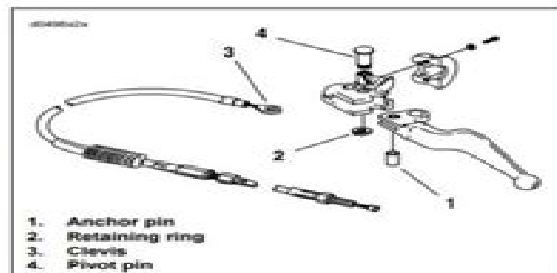
Figure 2-100. Clutch Cable Installation
