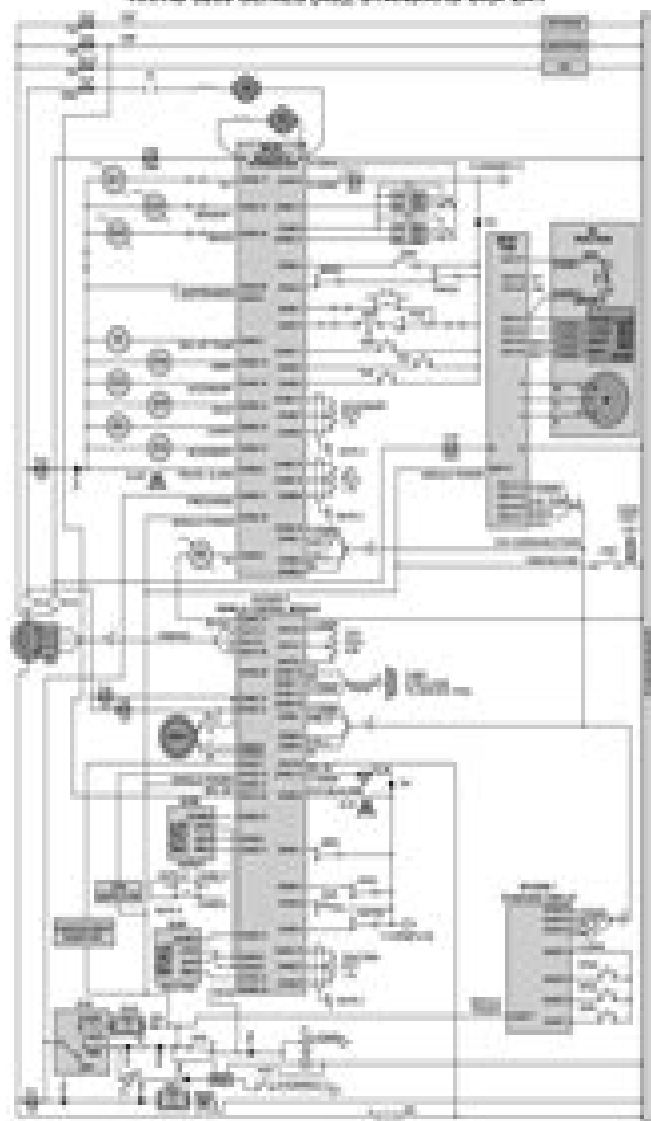
RRRD 1200 SERIES (AC), STANDARD DISPLAY
