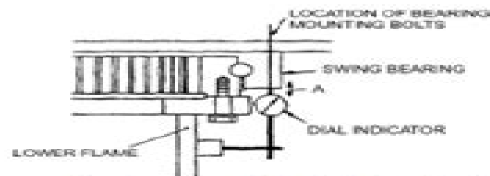
How to measure the axial play of swing bearing
