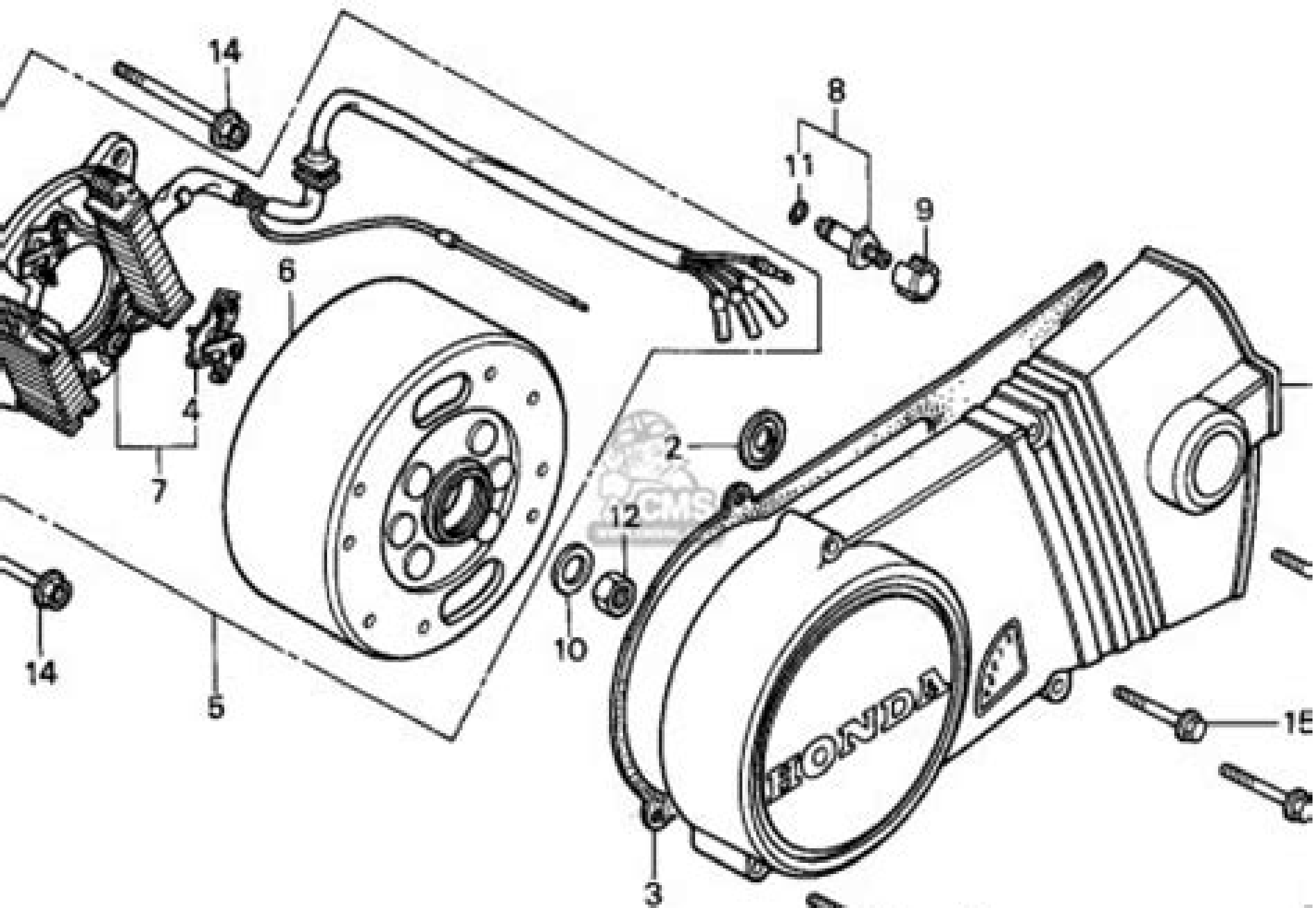
LEFT CRANKCASE COVER/ GENERATOR (1)
