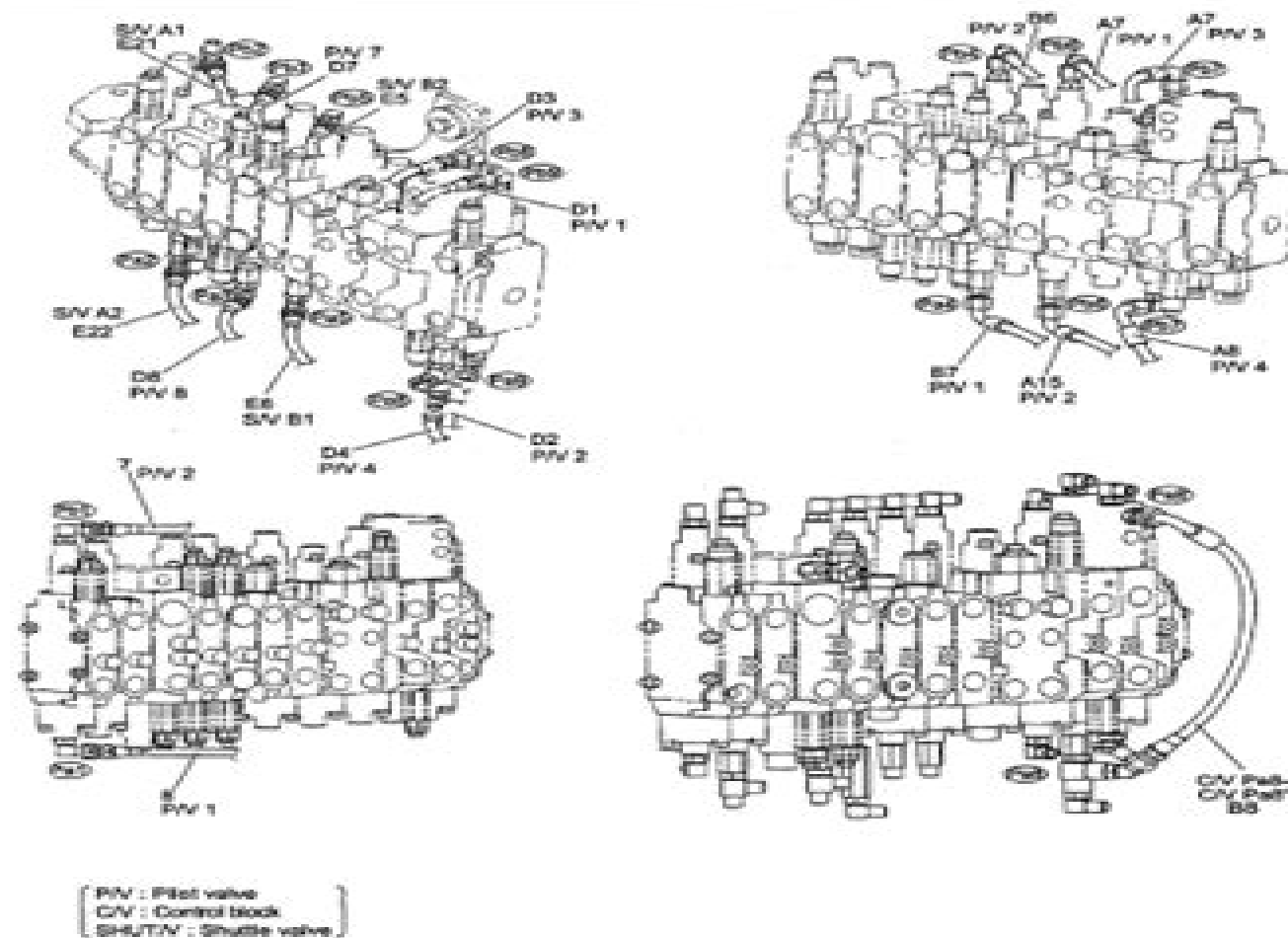
Fig. 33-24 Pilot hydraulic hose disconnection
