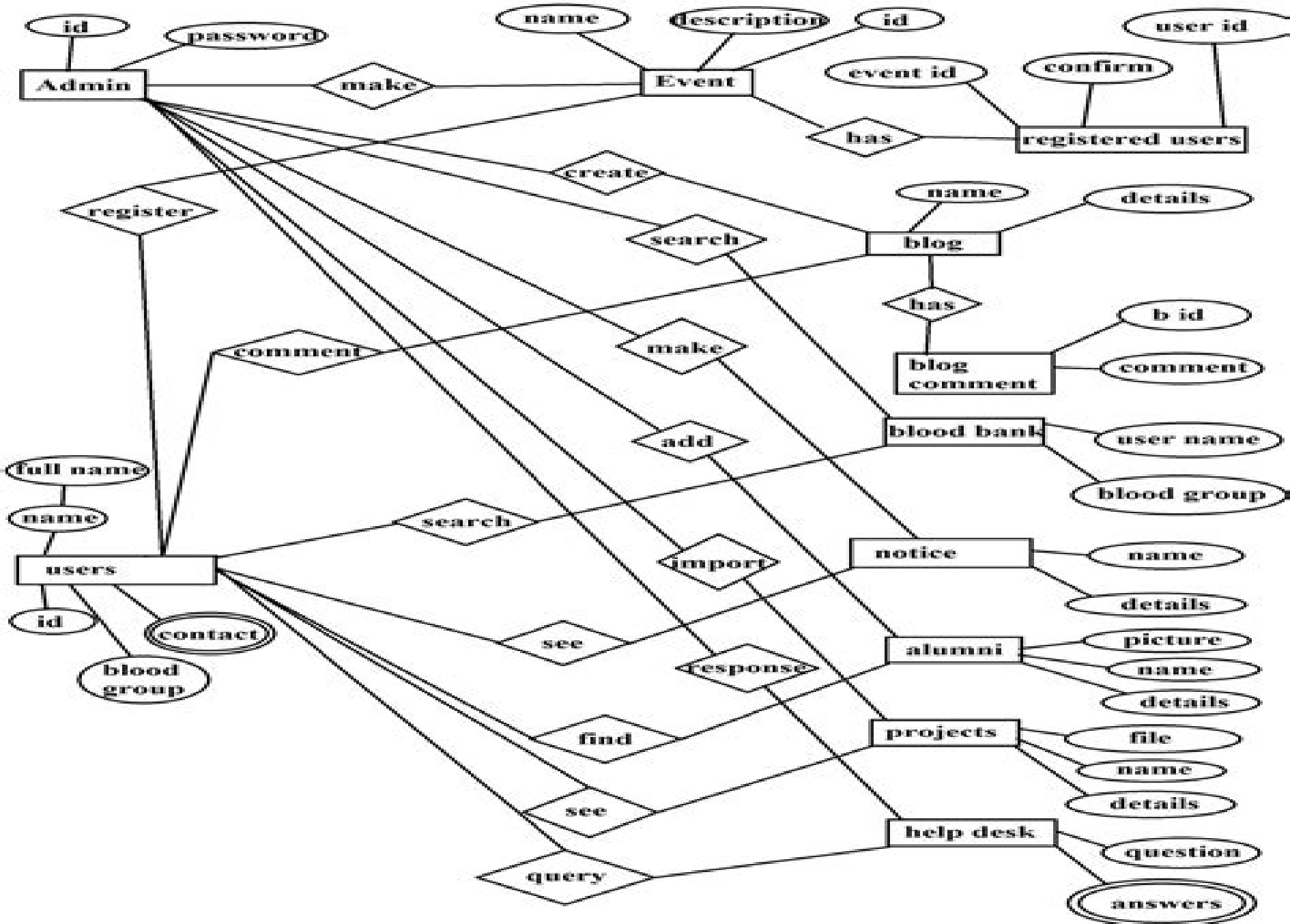
Fig: ER Diagram For Club Management System
