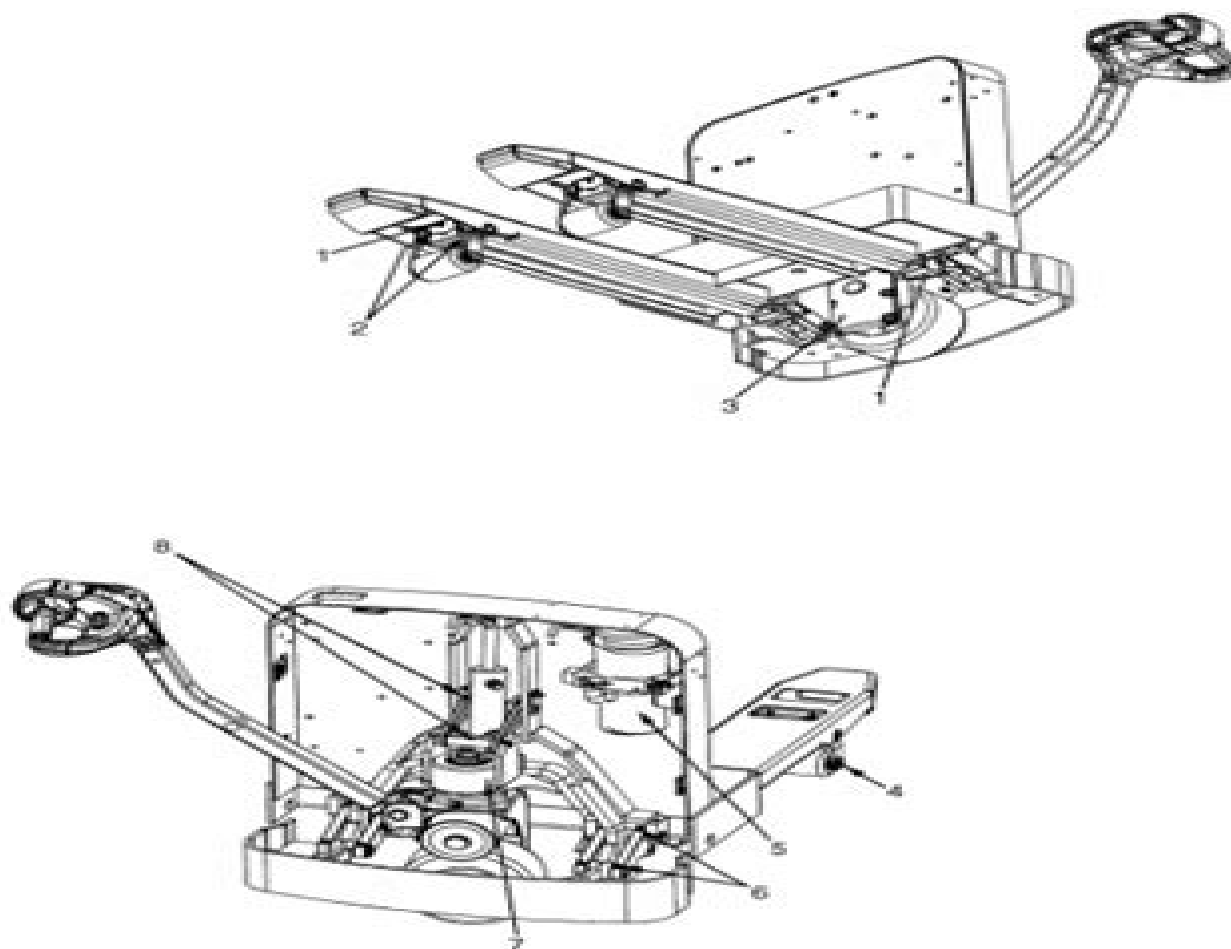
Figure 8. Lubrication Locations
