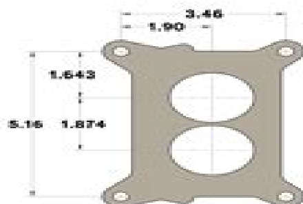
HOLLEY 2300 2-BBL
