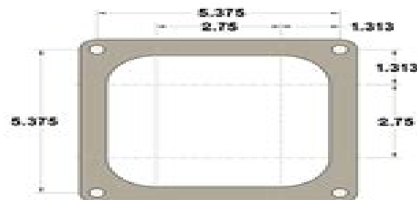
HOLLEY 4500 (DOMINATOR)
